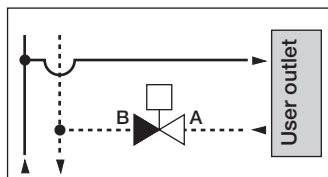
2-way installed on the return pipe
