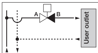
2-way installed on the flow pipe
