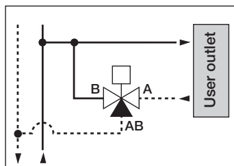
3-way installed on the return pipe with mixer position and ON/OFF operation
