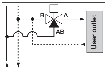
3-way installed on the flow pipe with diverter position and ON/OFF operation
